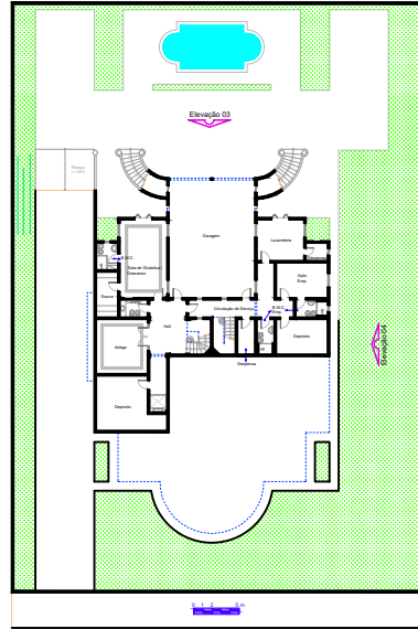
Subsolo A = 291,92 m 2
