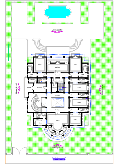
Superior A = 392,72 m 2
